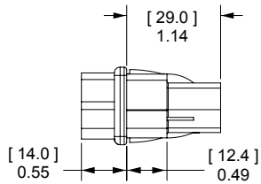
Short Depth - For Crimp Termination to Wire
