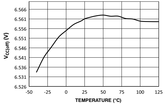
Figure 6. V CC(off) vs. Junction Temperature
