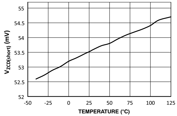
Figure 18. V_{ZCD(short)} vs. Junction Temperature
