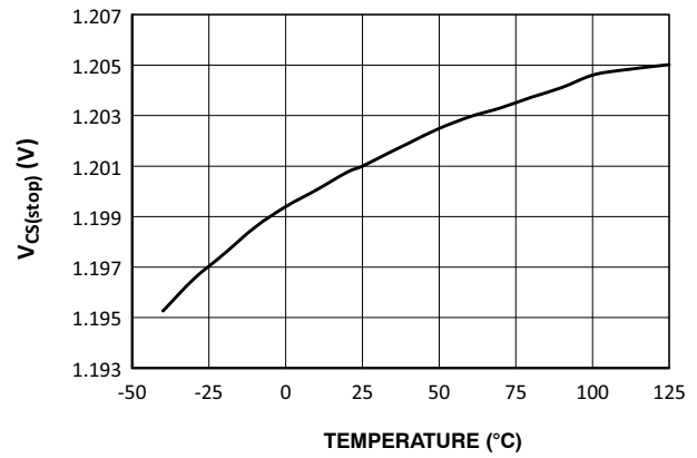
Figure 12. V_{CS(stop)} vs. Junction Temperature
