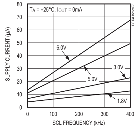
POWER-SUPPLY CURRENT vs. SCL FREQUENCY
