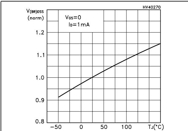
Figure 8. Normalized B_{V_{DS}} vs temperature
