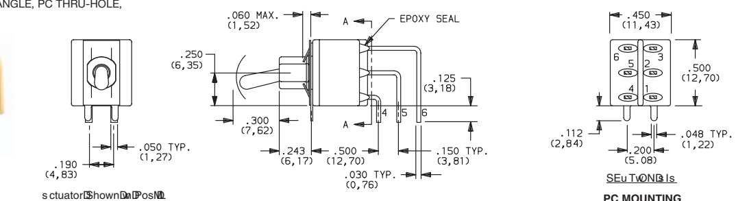
E201MD1AV2BE Vertical Actuation DPDT
