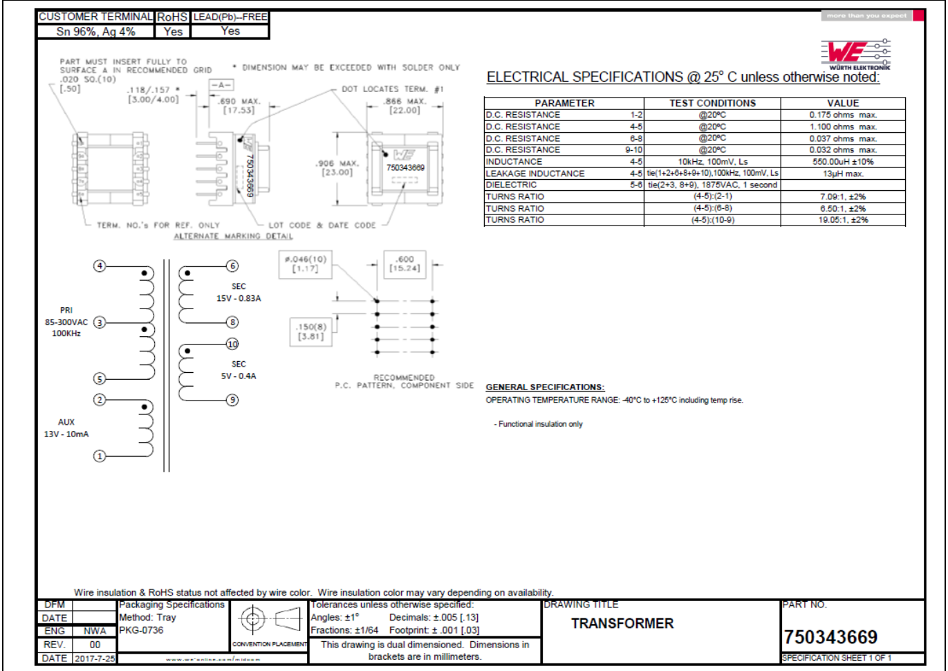
Figure 6 Transformer structure
