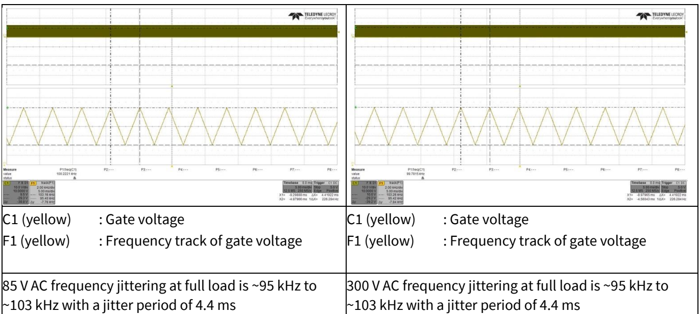
Figure 22 Frequency jittering
