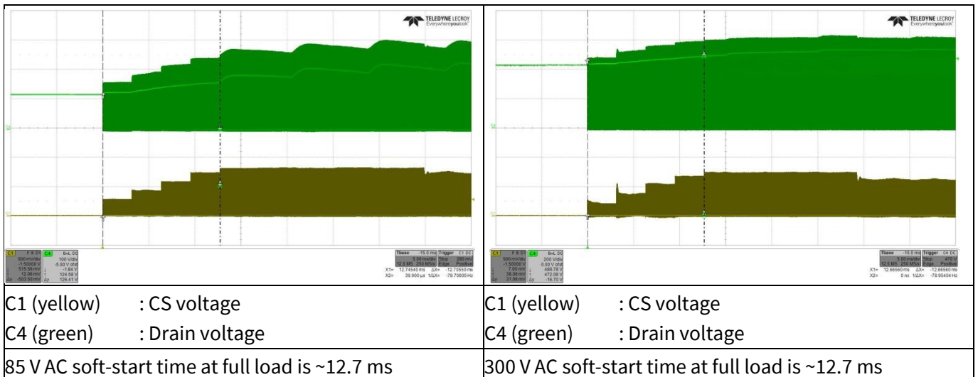
Figure 20 Soft-start
