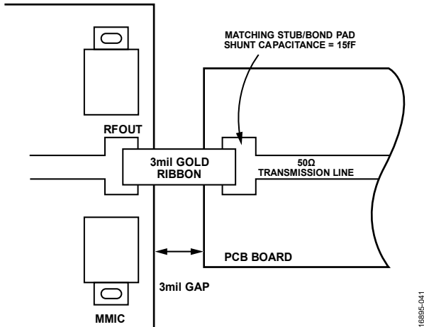
Figure 42. High Frequency Output Wideband Matching
