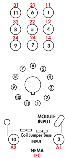
Wiring Diagram Top View
