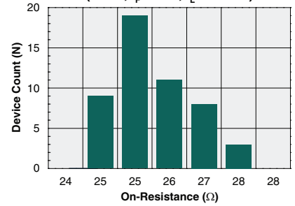
Typical On-Resistance Distribution (N=50, I_F=0\text{mA} , I_L=100\text{mA} )
