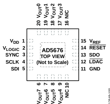
Figure 7. 20-Lead LFCSP Pin Configuration
