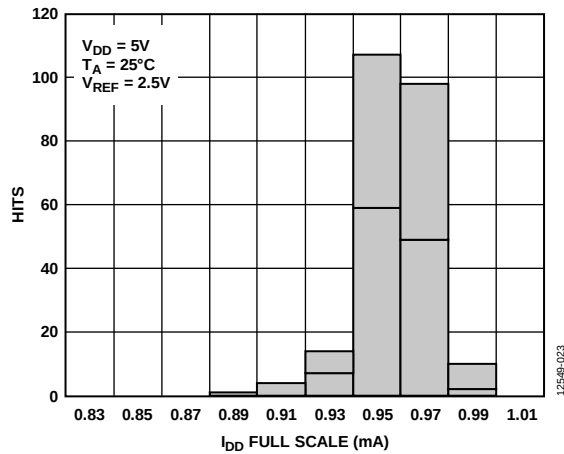
Figure 21. I_{DD} Histogram with External Reference
