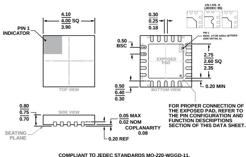
Figure 54. 20-Lead Lead Frame Chip Scale Package [LFCSP] 4 mm × 4 mm Body and 0.75 mm Package Height (CP-20-8)
