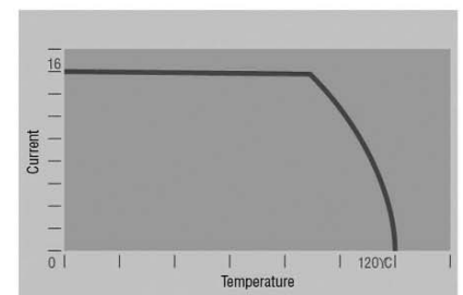
1.5mm², pre-tinned brass terminal. Test has been performed in ambient temperature
