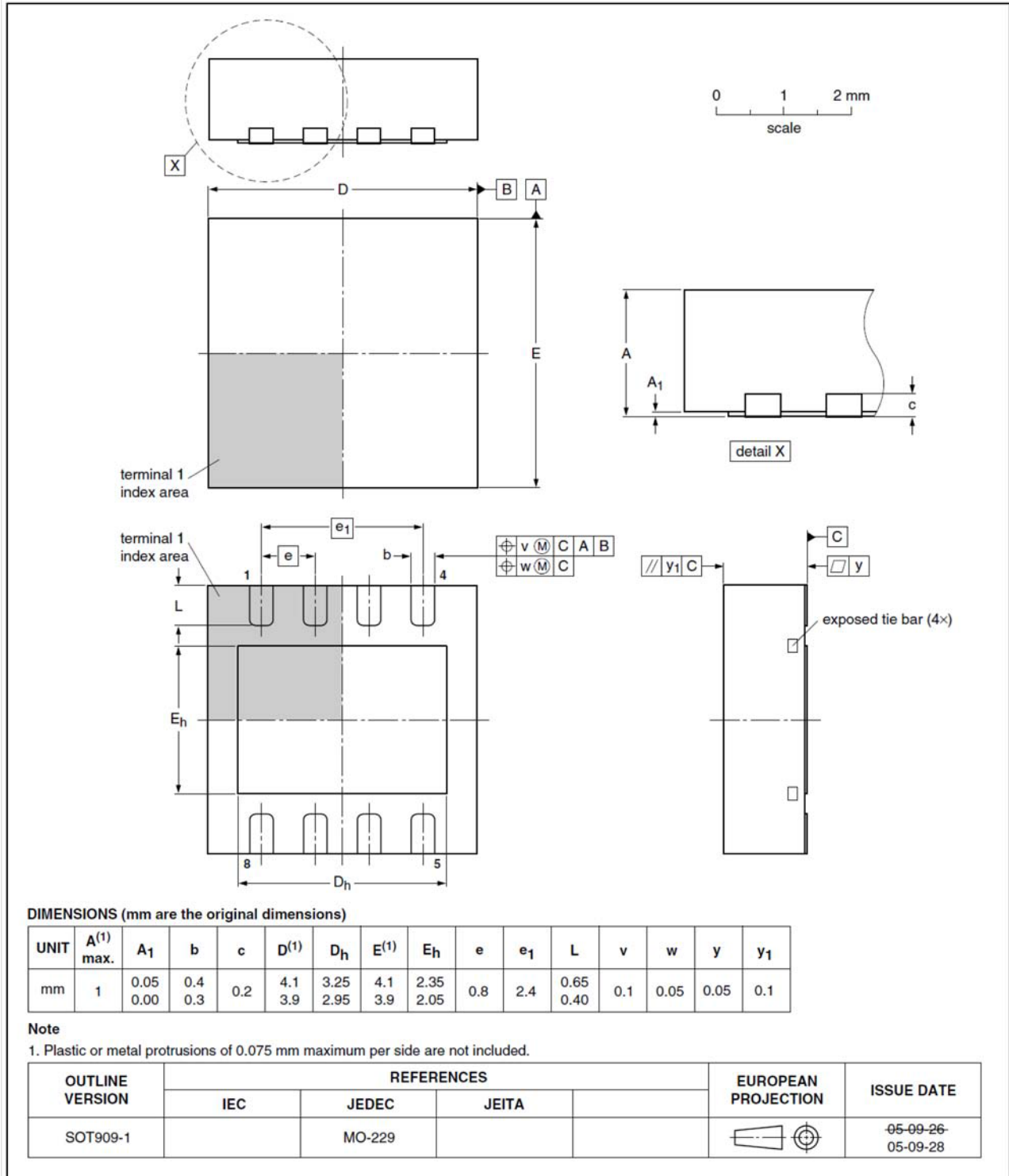
Fig 7. Package outline SOT909-1
