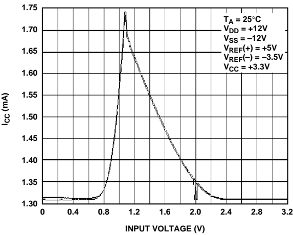
Figure 18. Supply Current vs. Digital Input Voltage
