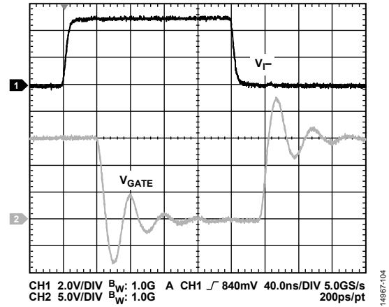
Figure 7. V_{I-} to V_{GATE} Waveform for 2 nF Load, 0 Ω Series Gate Resistor, V_{DD2} = 15\text{ V}
