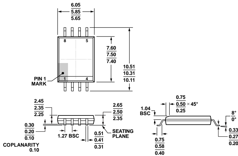
Figure 32. 8-Lead Standard Small Outline Package, with Increased Creepage [SOIC_IC] Wide Body (RI-8-1)
