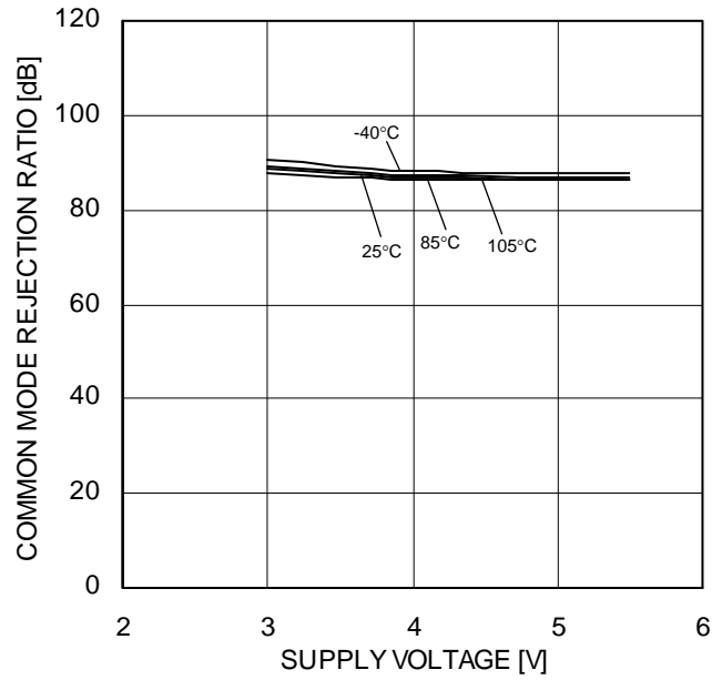
Figure 19. Common Mode Rejection Ratio – Supply Voltage
