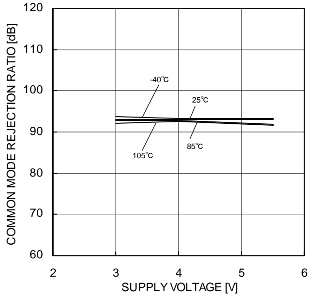
Figure 65. Common Mode Rejection Ratio – Supply Voltage
