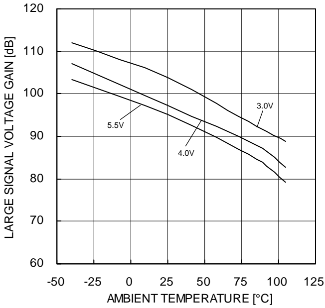
Figure 64. Large Signal Voltage Gain – Ambient Temperature
