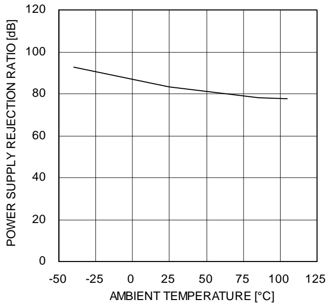
Figure 67. Power Supply Rejection Ratio – Ambient Temperature
