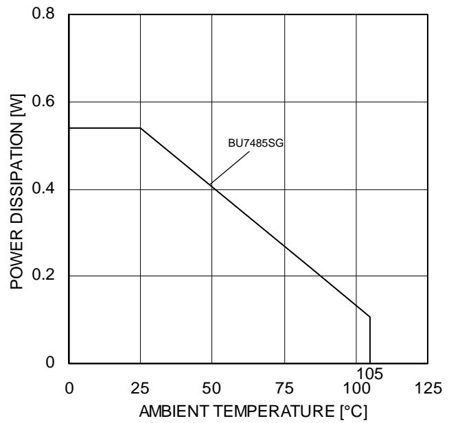
Figure 3. Derating curve
