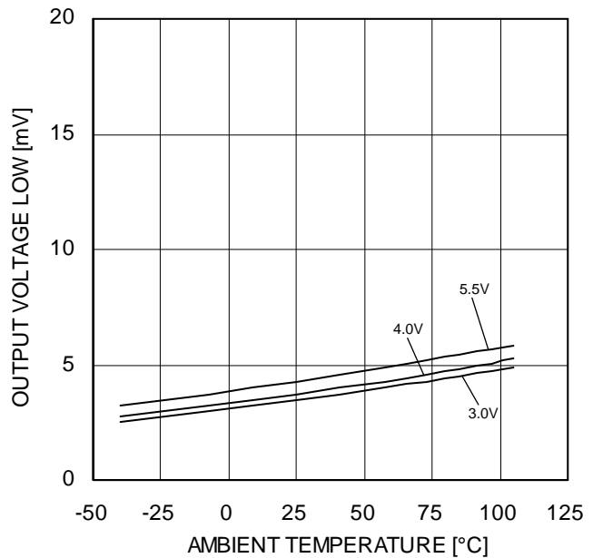
Figure 9. Maximum Output Voltage Low – Ambient Temperature (RL=10kΩ)
