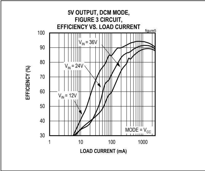
Figure 5. MAX17543 5V Output Efficiency (DCM Mode)
