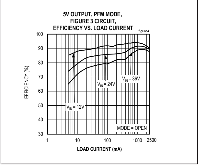
Figure 4. MAX17543 5V Output Efficiency (PFM Mode)
