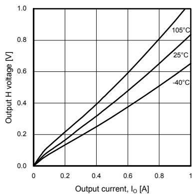
Figure 8. Output H Voltage (Temperature Characteristics)
