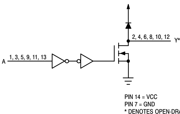
Figure 2. Logic Diagram
