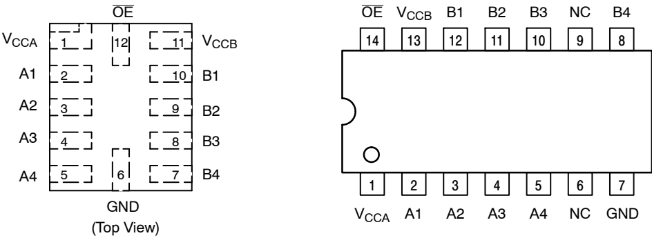
Figure 1. Pin Assignments
