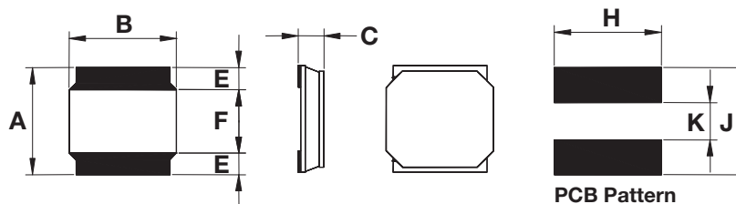
PCB Pattern
