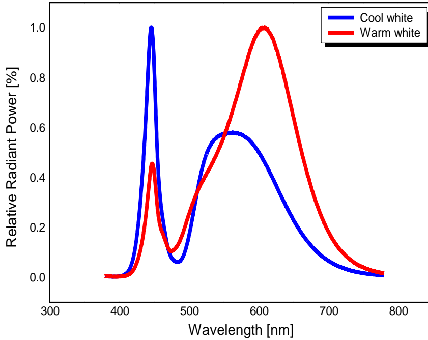
Fig 1. Color Spectrum, T_a = 25^\circ\text{C} , I_F = 500\text{mA} , \text{RH}30\%
