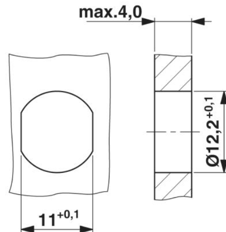
Mounting cut-out
