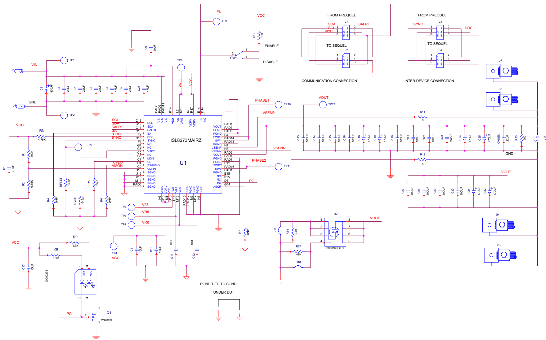
FIGURE 5. SCHEMATIC
