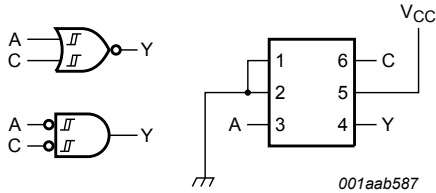
Figure 9. 2-input NOR gate or 2-input AND gate with both inputs inverted
