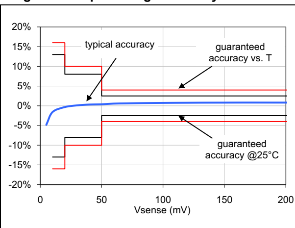
Figure 3. A1 pin voltage accuracy vs. Vsense
