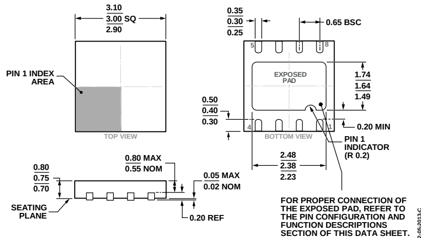
Figure 65. 8-Lead Lead Frame Chip Scale Package [LFCSP] 3 mm × 3 mm Body and 0.75 mm Package Height, Dual Lead (CP-8-3)
