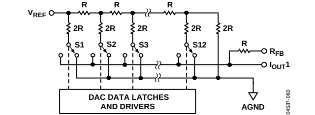
Figure 43. AD5452 Simplified Ladder
