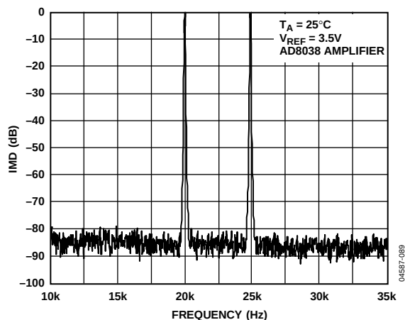
Figure 40. Narrow-Band IMD, f_{OUT} = 20\text{ kHz} , 25 kHz, Clock = 1 MHz
