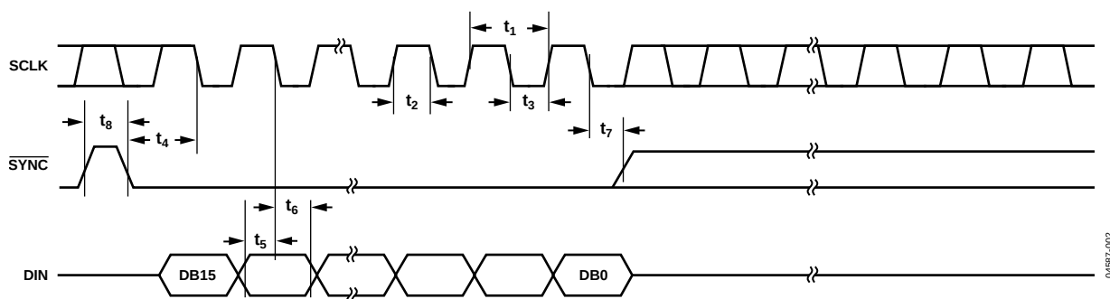
Figure 2. Timing Diagram
