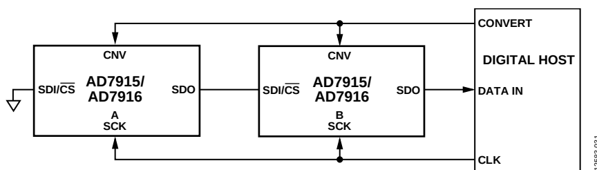
Figure 42. Chain Mode Without Busy Indicator Connection Diagram
