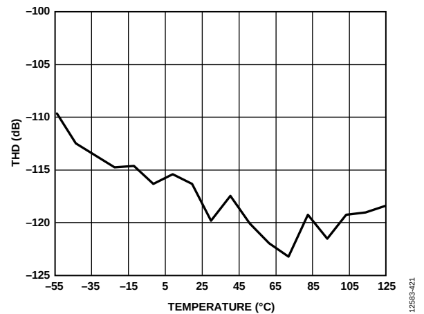
Figure 20. THD vs. Temperature
