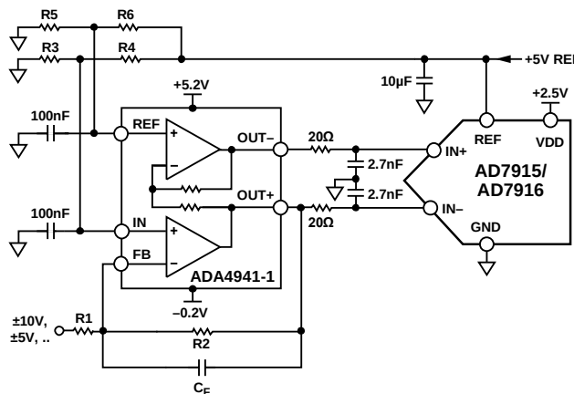
Figure 32. Single-Ended to Differential Driver Circuit
