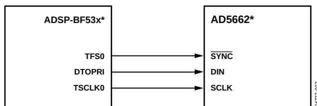
Figure 37. AD5662 to Blackfin ADSP-BF53x Interface
