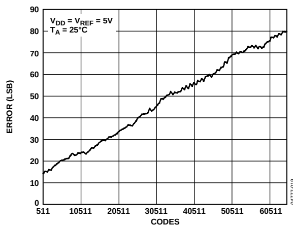
Figure 6. Typical Total Unadjusted Error Plot
