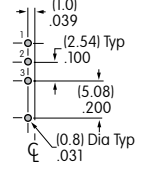
V1 Terminals
