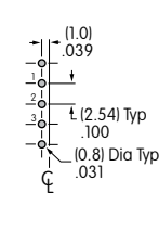
B1 Terminals
