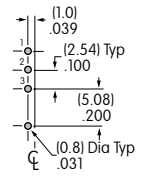
V1 Terminals
