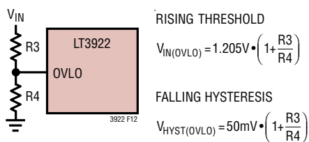
Figure 12. OVLO Threshold and Hysteresis Voltages
