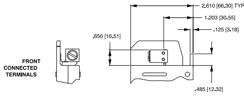
BOX TYPE WIRE CONNECTORS
