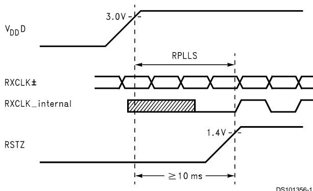
FIGURE 1. FPD85308 (Receiver) Phase Lock Loop Set Time
