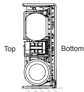
Fig. 4: Mounting on the right side
