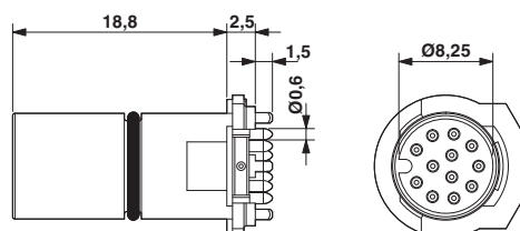
M12 plug, straight
