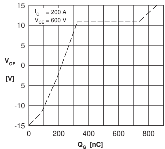
Fig. 6 Typ. turn-on gate charge -15/+15V
