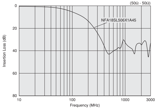
NFA18SL_X
