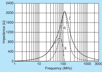
BLM21BD182SN1
