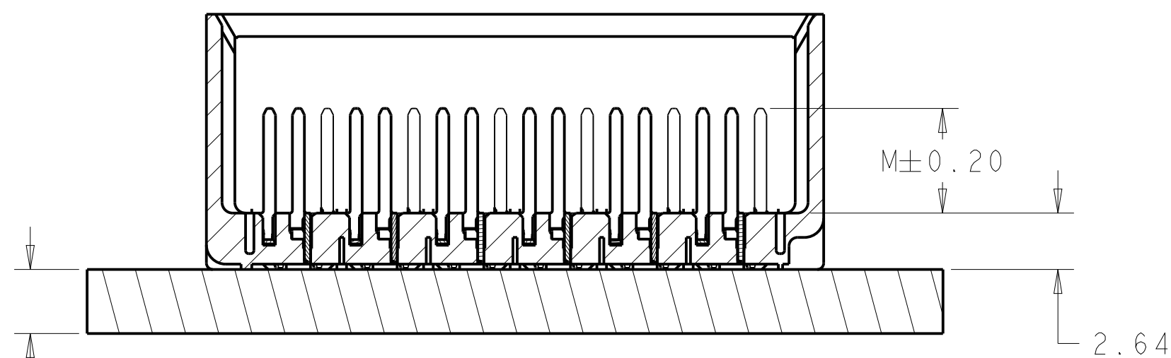
SECTION Z-Z
