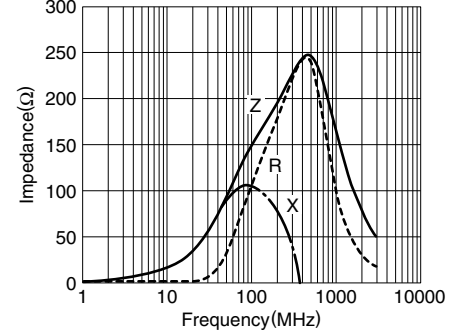
MPZ1608Y151B
