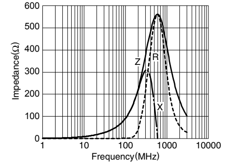
MPZ1608D101B
