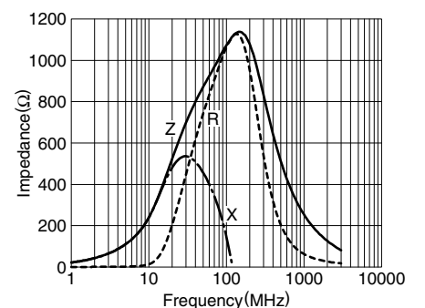
MPZ1608S102A
